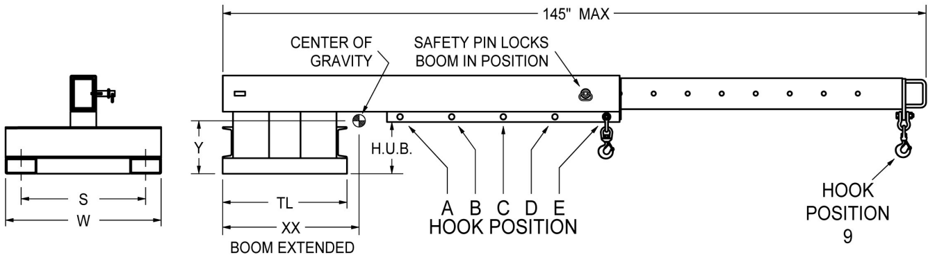
"JLT" Series Telescoping Jib Lift
